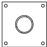
2X 6" X 6" X .25" FLANGE MOUNTING PLATE WITH 4 5/8" MOUNTING HOLES
