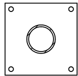
2X 6" X 6" X .25" SQUARE FLANGE MOUNTING PLATE WITH 4 Ø 3/8" MOUNTING HOLES
