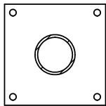
2X 6" X 6" X .25" SQUARE FLANGE MOUNTING PLATE WITH 4 \varnothing 5/8" MOUNTING HOLES
