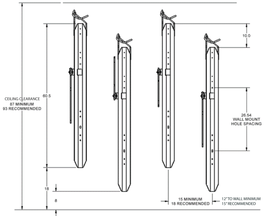
Product shown 6106 with pivoting lock bar
